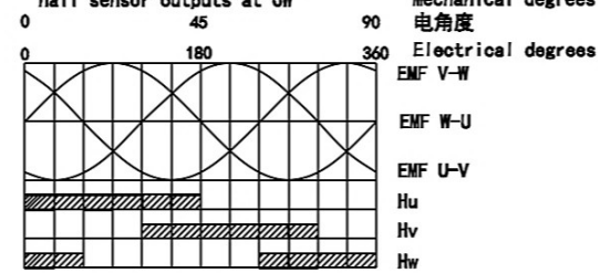
线反电势与霍尔相位关系图 (顺时针) Relation between phase EMF's and hall sensor outputs at CW
